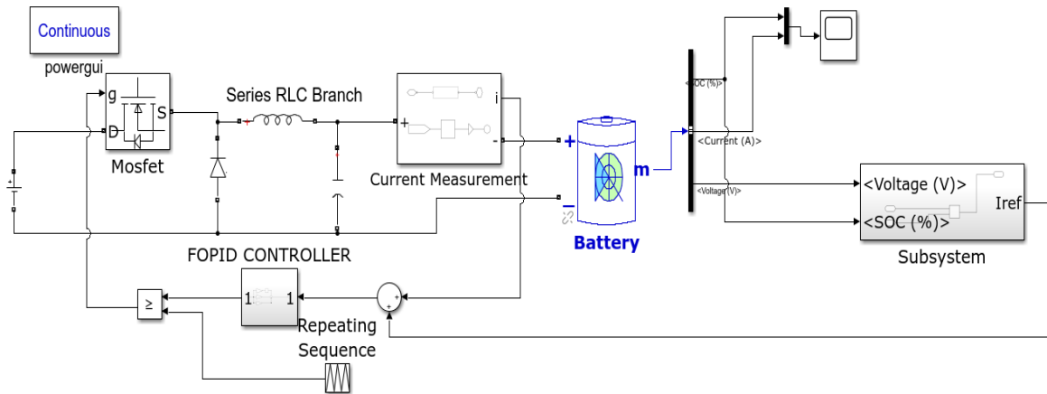
Fig.7. Schematic of five-level charging systems using FOPID controller in MATLAB/SIMULINK.
