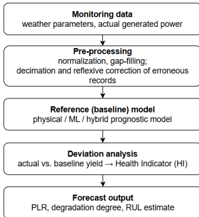
Fig. 3. Information-processing pipeline in PV-panel degradation forecasting methods.
