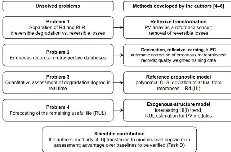
Fig. 4. Correspondence between the unsolved degradation problems and the methods developed earlier by the authors [4–6].
