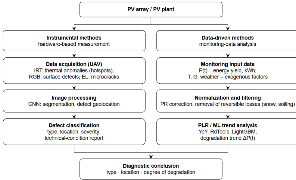
Fig. 1. Information extraction and processing scheme in PV-panel degradation diagnostic methods.
