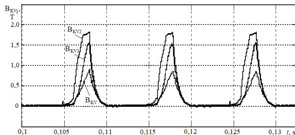
Fig. 4. Temporal dependencies of magnetic induction for elements #2, #3, and continuous stator tooth. 4
